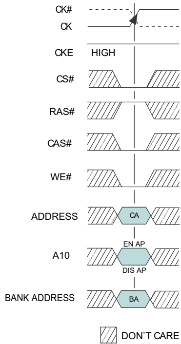
FIGURE 12 – WRITE COMMAND
