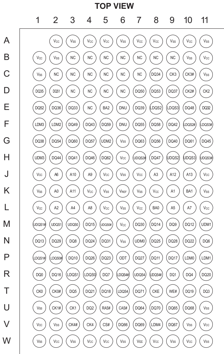
FIGURE 3 - PIN CONFIGURATION
