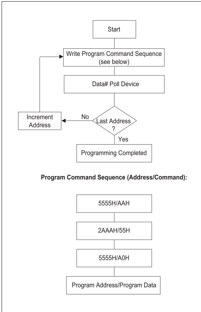
Figure 2 – Programming Algorithm
