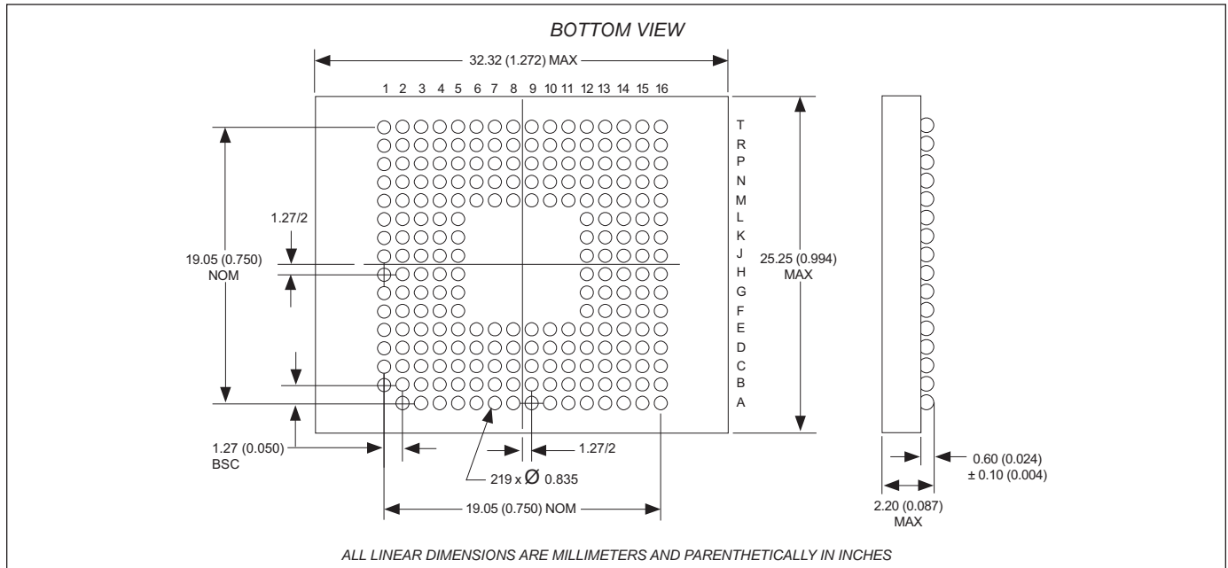
Figure 1 – Package Dimension: 219 Plastic Ball Grid Array (PBGA)
